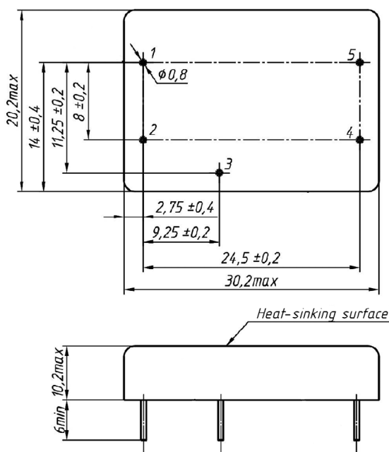
Figure 5. VFA2,5 version.
