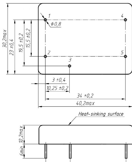
Figure 7. VFA5 version.
