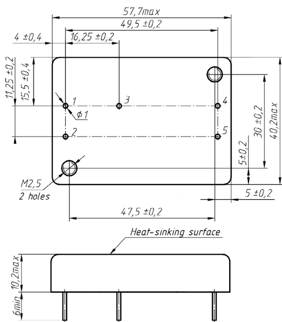
Figure 11. VFA20 version.
