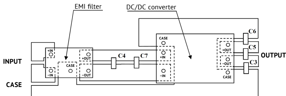
Figure 1. VFA layout.
