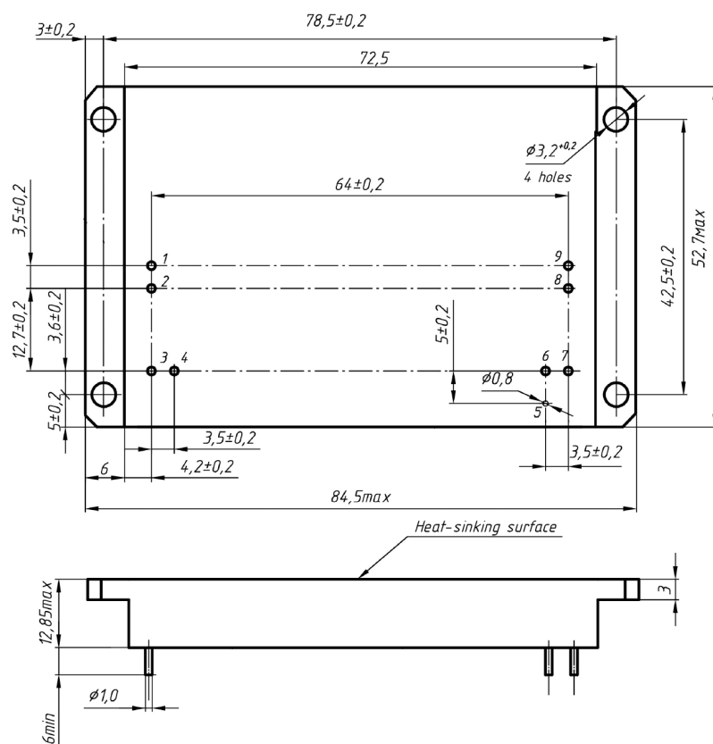
Figure 13. VFA2U, VFA4,5U version.
