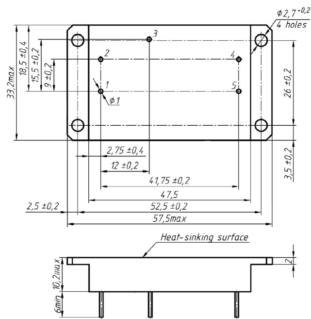
Figure 10. VFA10U version.
