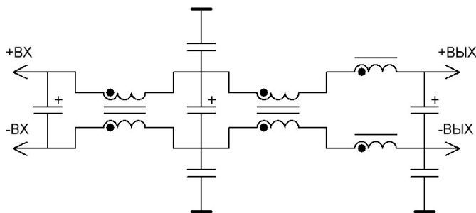
Figure 4. VFA typical connection diagram.
