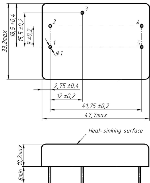
Figure 9. VFA10 version.
