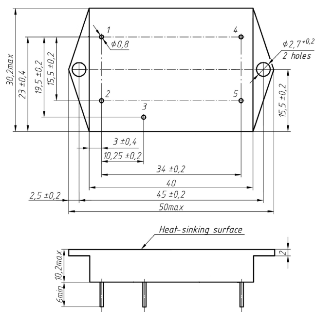
Figure 8. VFA5U version.
