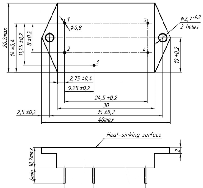
Figure 6. VFA2,5U version.
