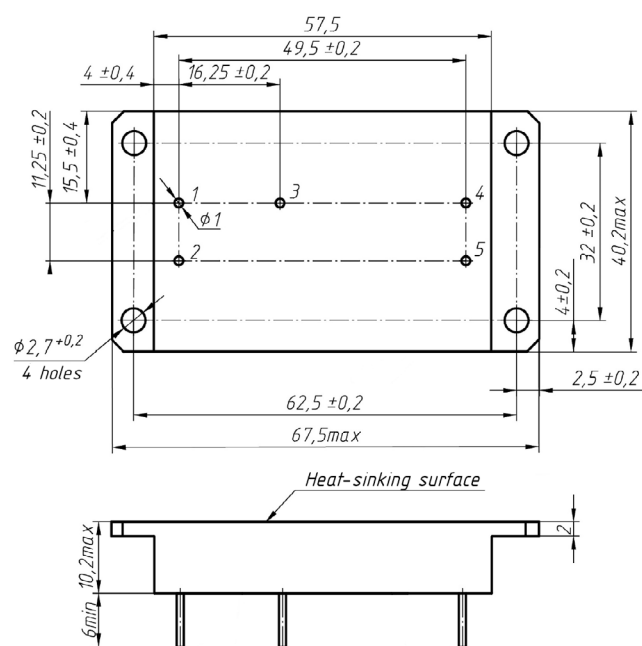
Figure 12. VFA20U version.
