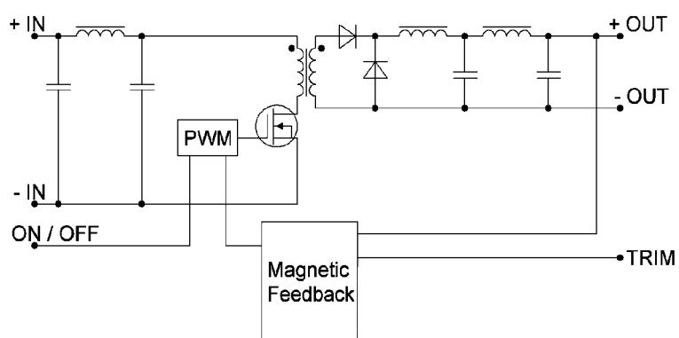
Figure 1. Design topology.
