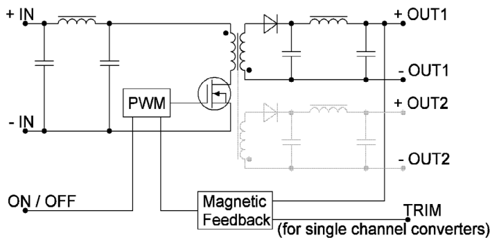
Figure 1. Design topology.
