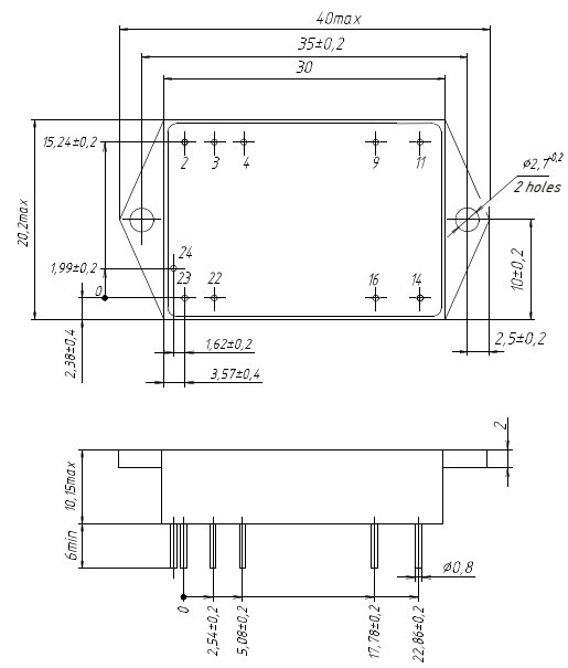
Figure 9 (b). Dual-output models.
