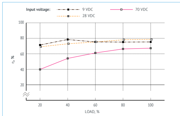
Figure. 6 (a). Efficiency of VDV8-1E12.
