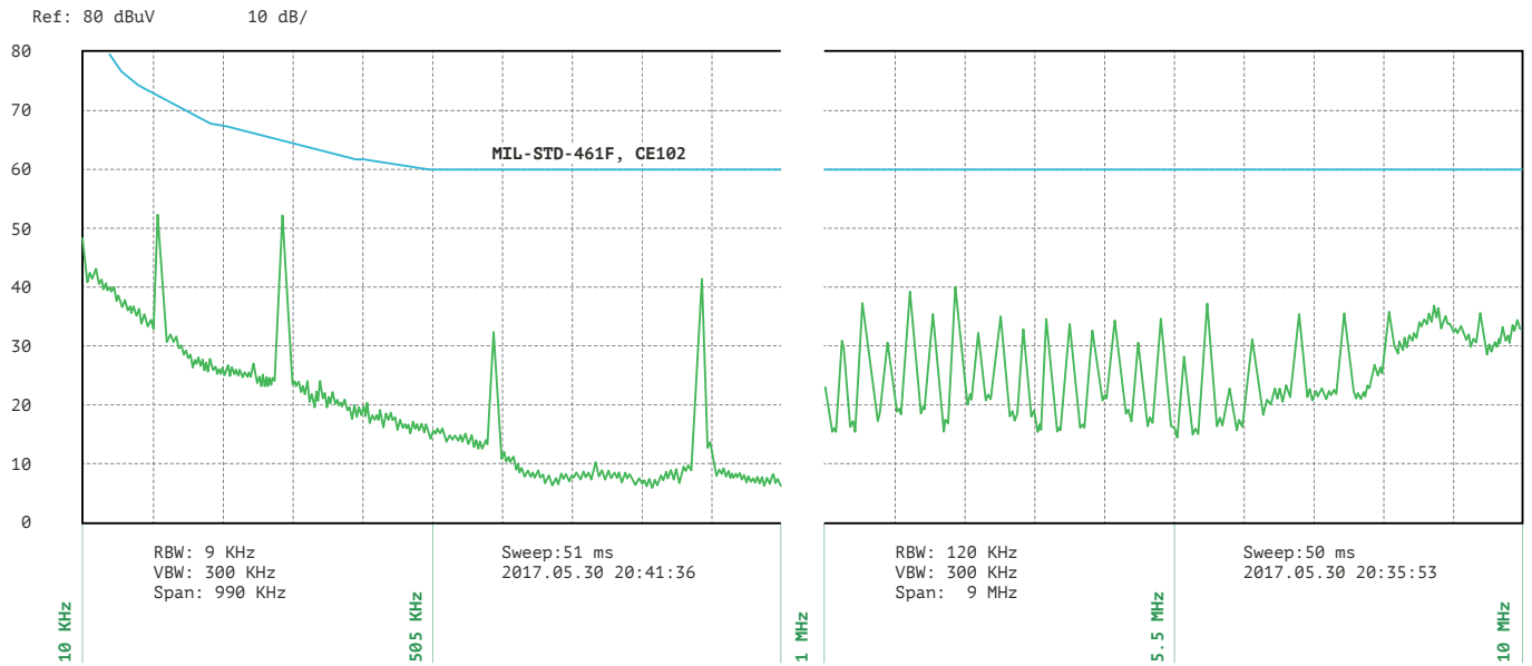
Figure 8. Spectrogram of VDV8 with typical connection diagram.
