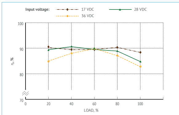
Figure 7. Efficiency of VDV400-1V28.
