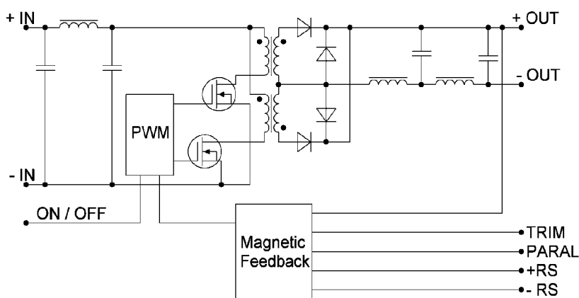
Figure 1. Design topology.
