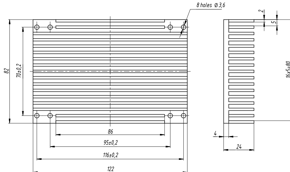
Figure 11 (b).752695.008-01.
