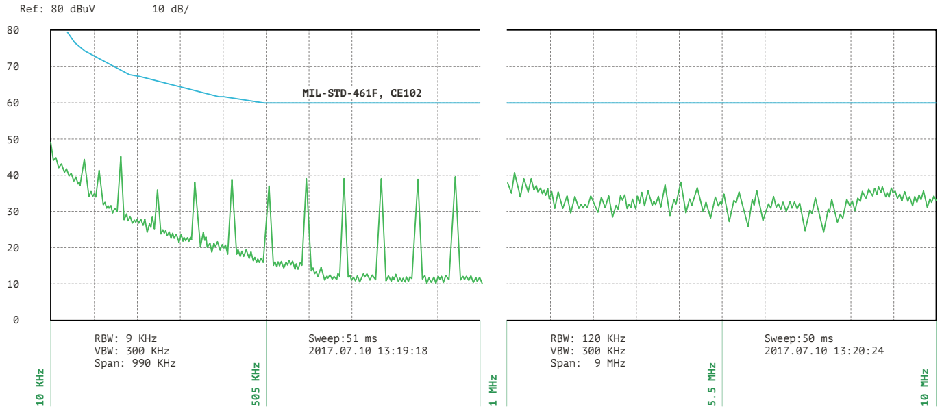
Figure 9. Spectrogram of VDV500-1V28 with typical connection diagram.
