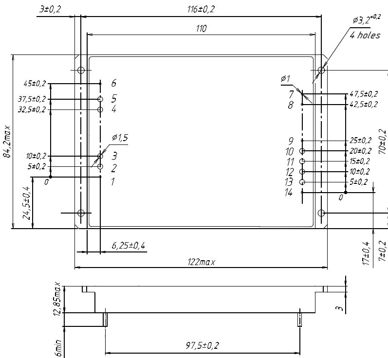
Figure 10. Single-output models.
