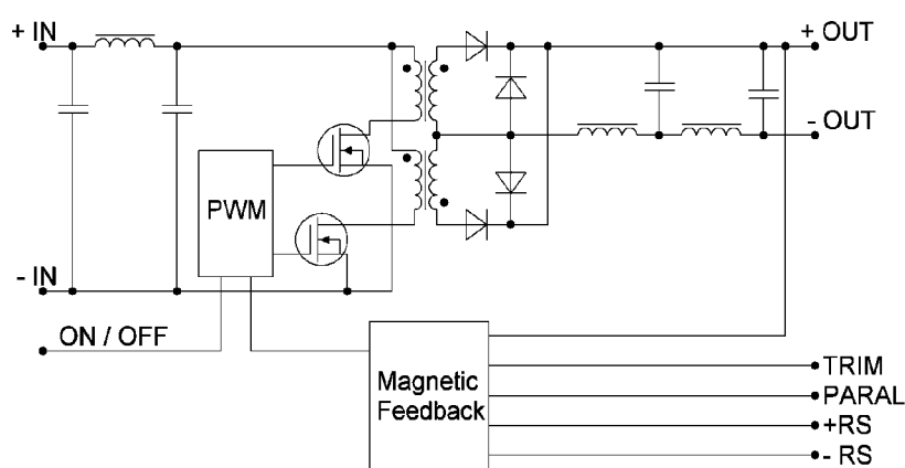
Figure 1. Design topology.
