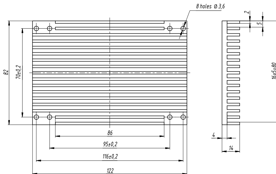
Figure 11 (a).752695.008.
