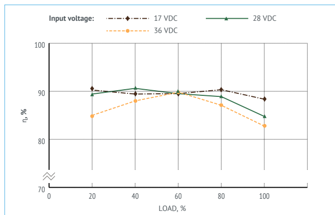
Figure 7. Efficiency of VDV400-1V28.
