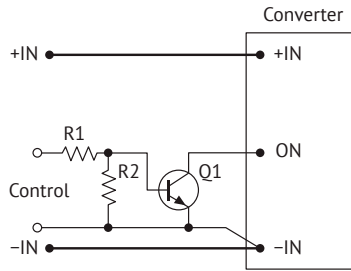
Figure 3 (b). ON/OFF control by bipolar transistor.
