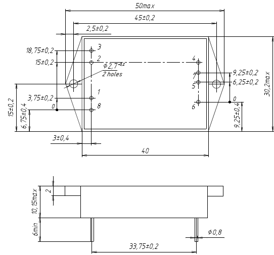
Figure 9 (b). Dual-output models.
