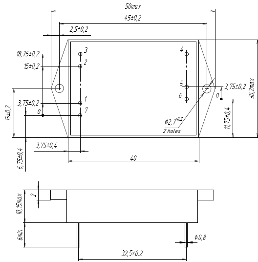
Figure 9 (a). Single-output models.
