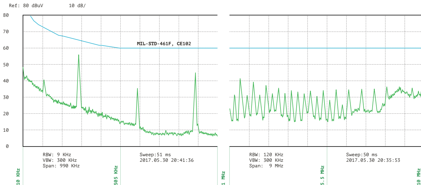
Figure 8. Spectrogram of VDV12 with typical connection diagram.
