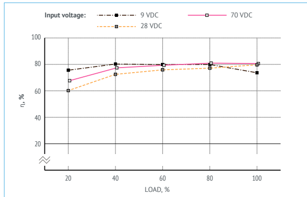
Figure. 6 (a). Efficiency of VDV12-1E12.
