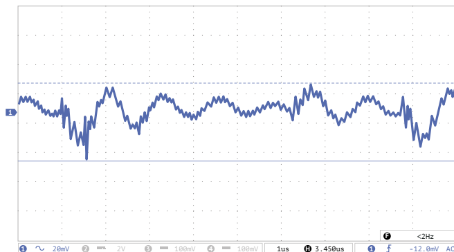
Figure 8 (c). Oscilloscope chart of output voltage ripple.
