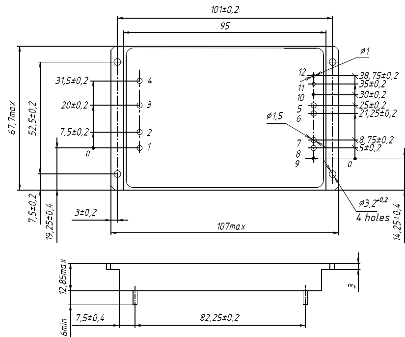
Figure 10. Single-output models.
