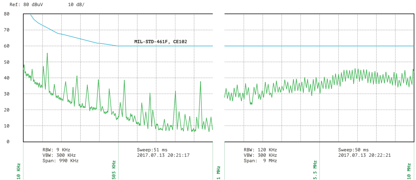
Figure 9. Spectrogram of VDV(HV)160-1M05 with typical connection diagram.
