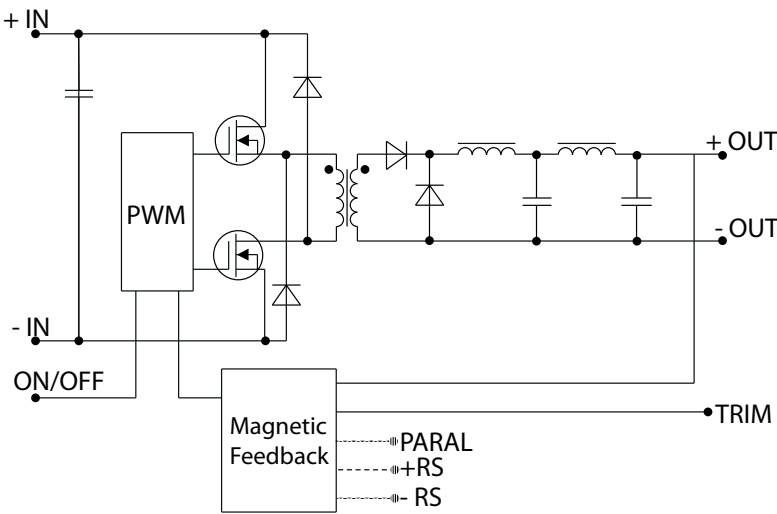
Figure 1. Design topology.
