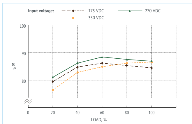
Figure 7. Efficiency of VDV(HV)160-1M28.
