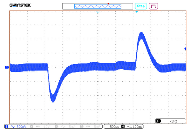
Figure 30. U_{OUT,NOM} transient deviation on 0,75...1 \cdot I_{OUT} change.
