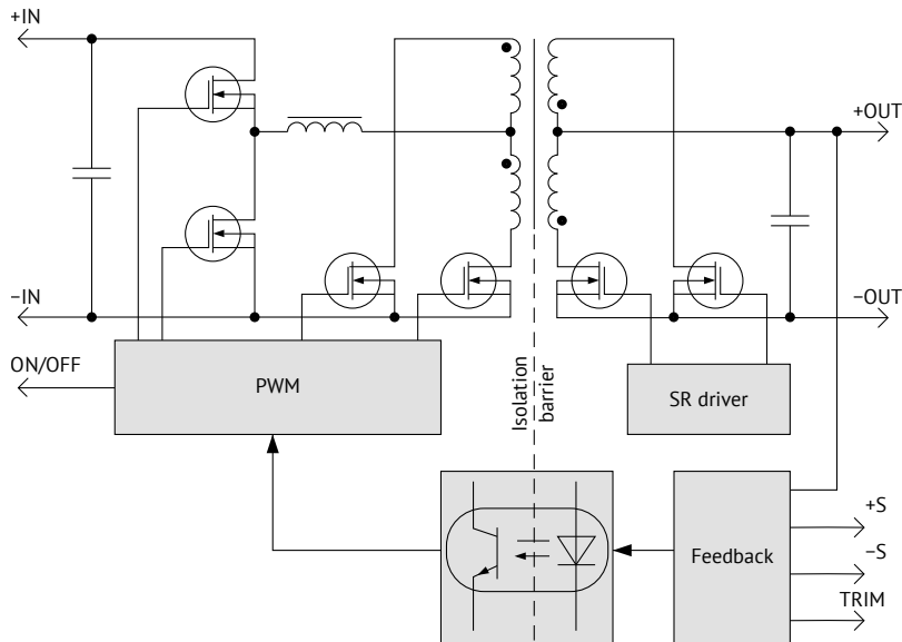
Figure 1. VDRW50 layout.
