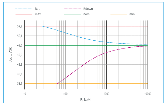
Figure 11. Chart for VDRW50N48.
