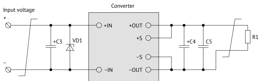
Figure 2. VDRW50 typical connection diagram.
