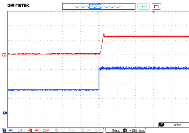
Figure 27. U_{OUT,NOM} stabilizing with Remote On/Off option (control signal).
