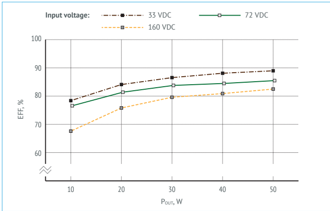
Figure 24. Efficiency.
