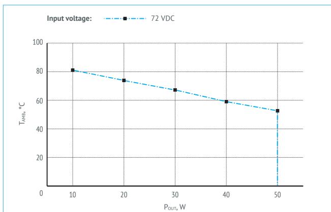
Figure 17. P_{OUT} vs T_{AMB} chart.
