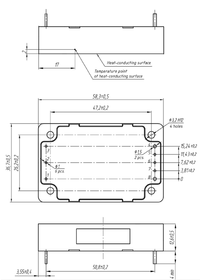
Figure 32. 1/4 Brick.
