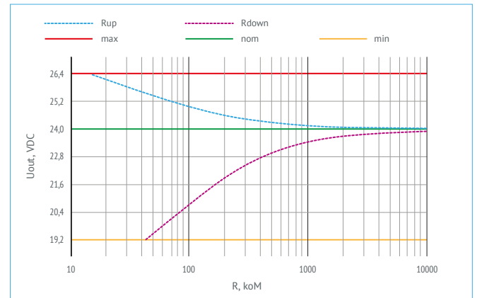
Figure 9. Chart for VDRW50N24.
