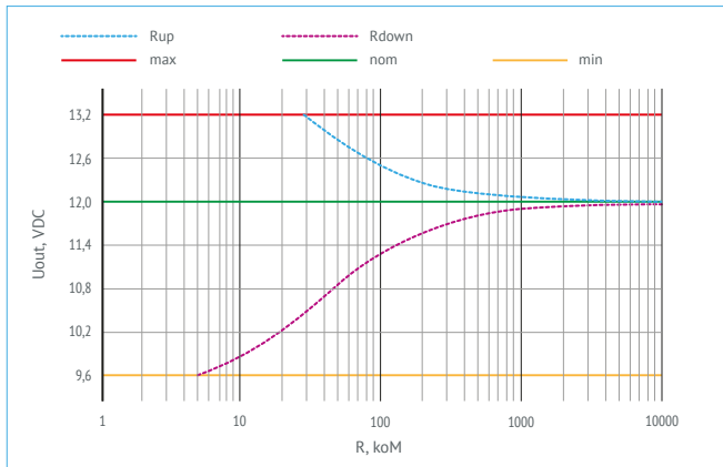
Figure 7. Chart for VDRW50N12.
