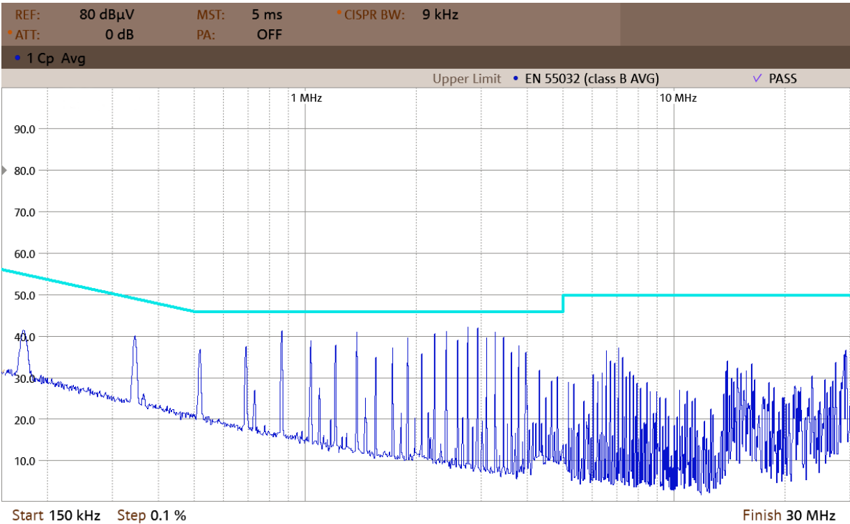
Figure 31. Spectrogram 0,15–30 MHz.
