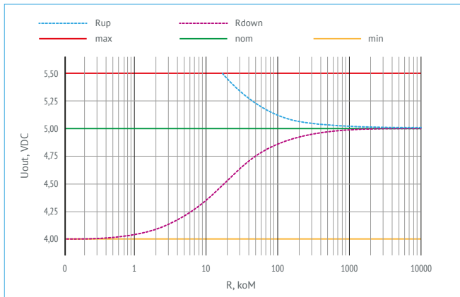
Figure 6. Chart for VDRW50N05.
