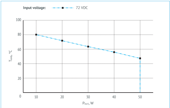
Figure 25. P_{OUT} vs T_{amb} chart.
