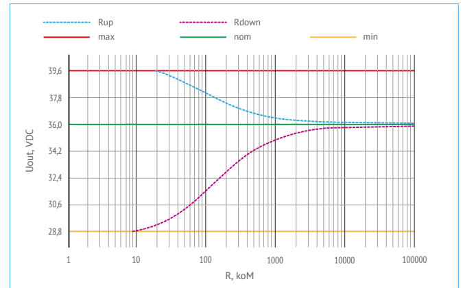
Figure 10. Chart for VDRW50N36.
