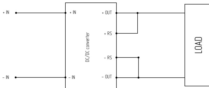
Figure 13. Typical connection diagram without external feedback application.
