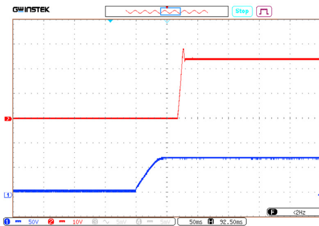
Figure 28. U_{OUT,NOM} stabilizing with U_{IN,NOM} .
