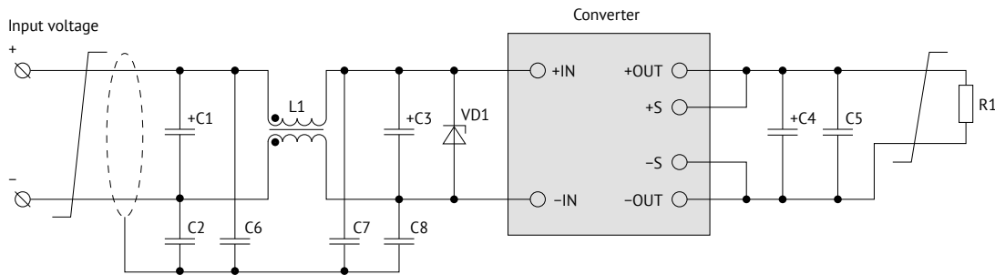
Figure 3. VDRW50 connection circuit for EN55032 Class B.
