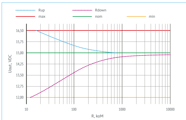
Figure 8. Chart for VDRW50N15.
