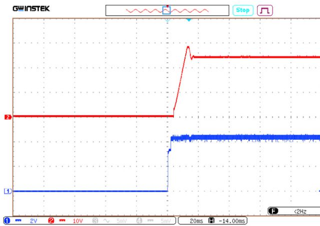
Figure 26. U_{OUT,NOM} stabilizing with Remote On/Off option (ON and -OUT pins connection).
