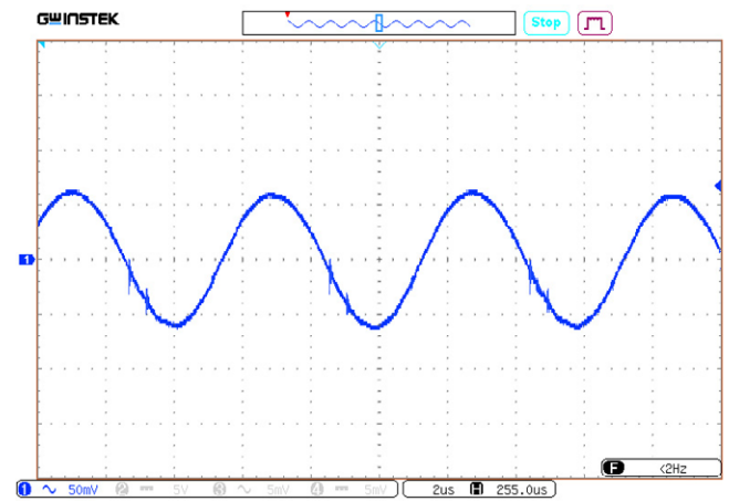
Figure 29. U_{OUT,NOM} ripple.
