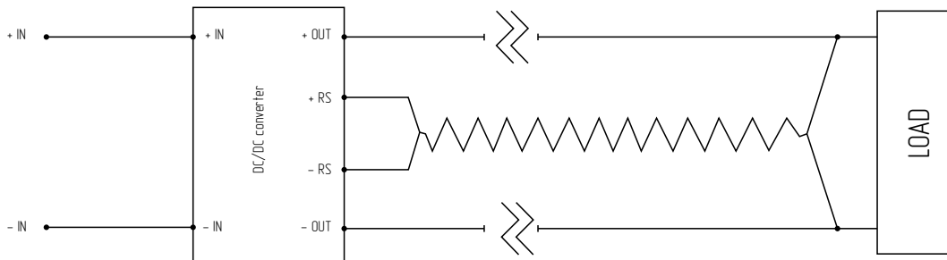
Figure 12. Typical connection diagram of external feedback application.
